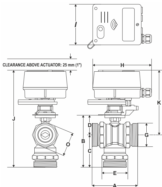
Fig. 3. M6061/M7061 + 3-way ball valve (see also Table 7)
