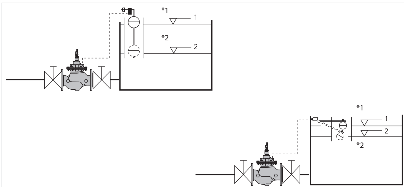
Fig. 1 Standard installation example for the filling valve
