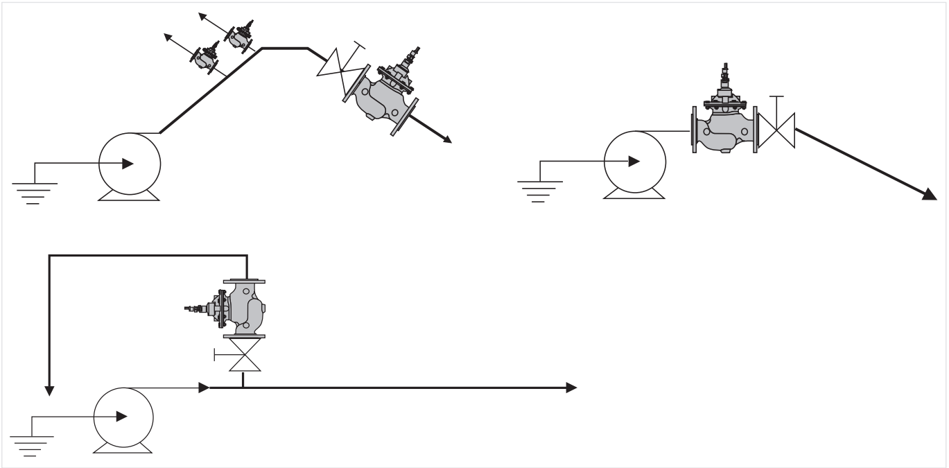
Fig. 1 Standard installation example for the pressure sustaining valve
