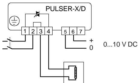
Figure 1 External input signal
