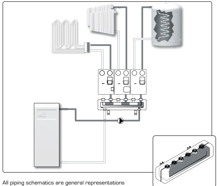
All piping schematics are general representations
